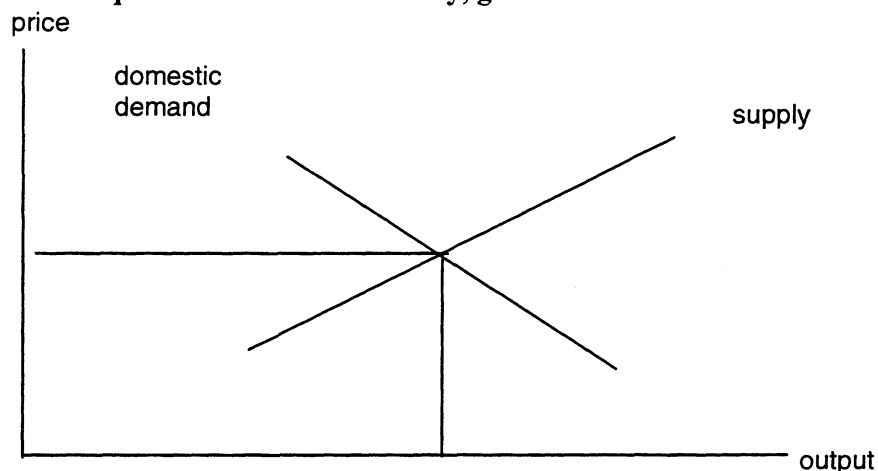
Figure 3-3 Partial equilibrium in the Electricity, gas and water sector
